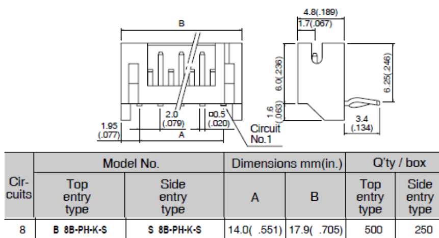
Fig.2 Pitch 2.0mm Port
